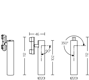
SK02 - directional spot faretto orientabile W 1
