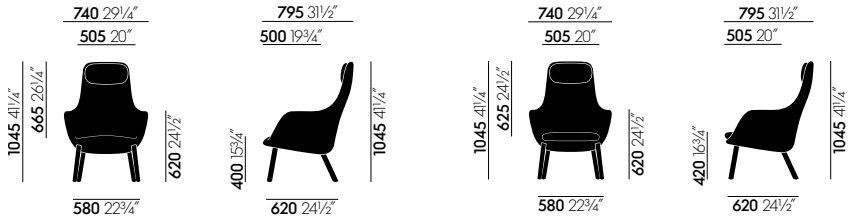
HAL Lounge Chair integrated cushion
